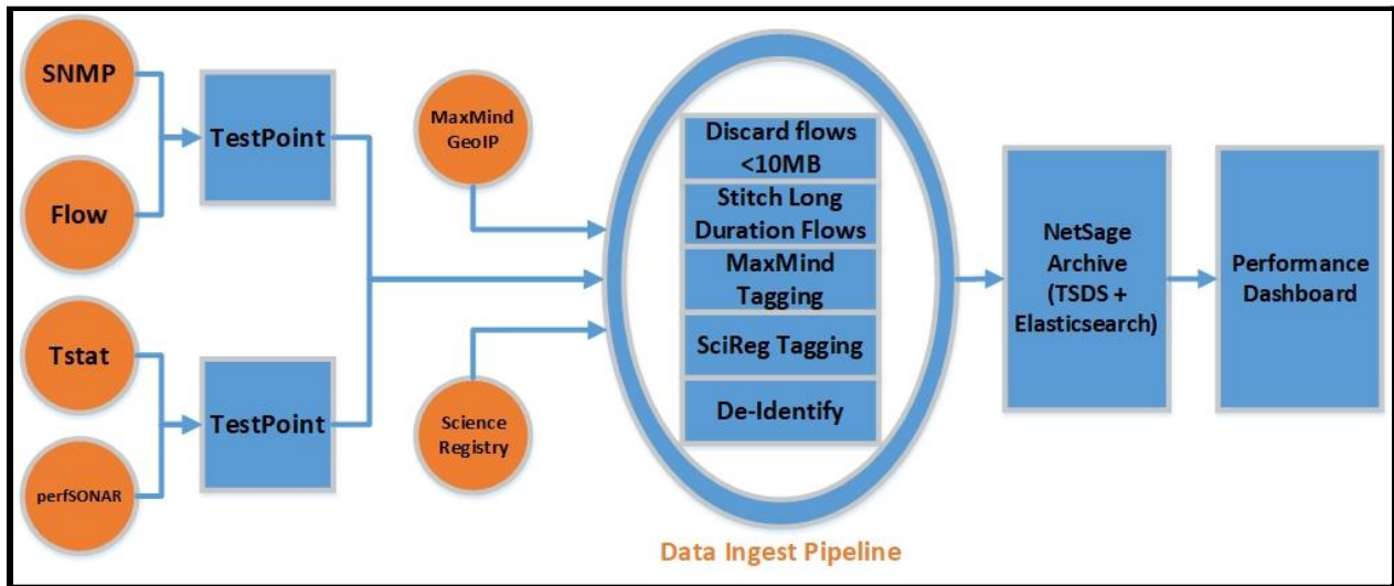
Figure 1: The NetSage logical architecture.
